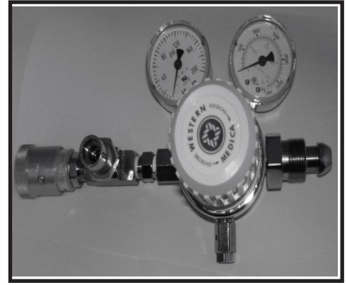
Adjustable, 0-200 PSI, Diaphragm 2" Gauges, Schrader Coupler & DISS
