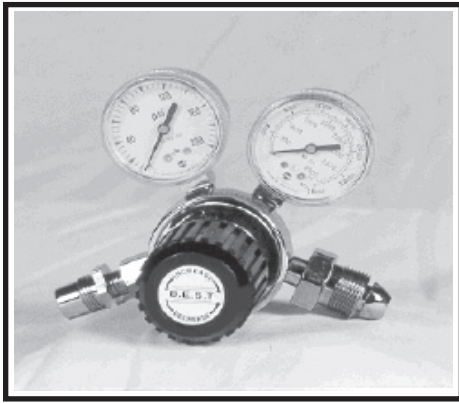
Adjustable, 0-200 PSI, Diaphragm 2" Gauges with DISS Outlet
